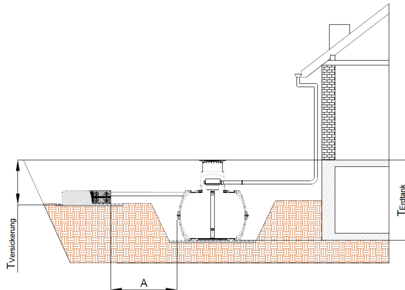
Figure 5: Installation situation: Distance to an upstream underground tank
