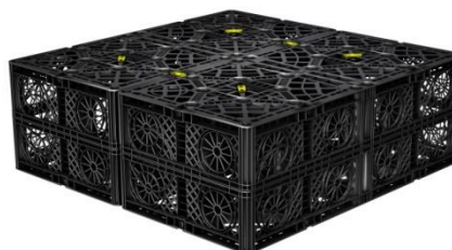
Figure 12: Vertical connection - EcoBloc connectors
