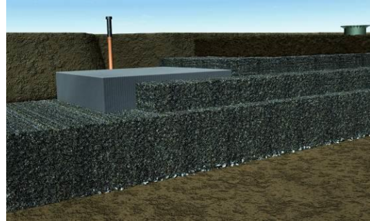
Figure 18: Backfilling the infiltration system
