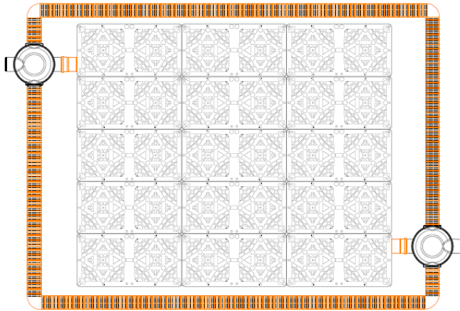
Figure 16: Partial drainage pipes circumferential
