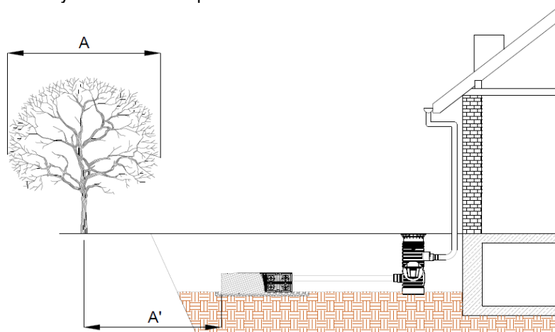
Figure 3: Installation situation: Distance to trees
