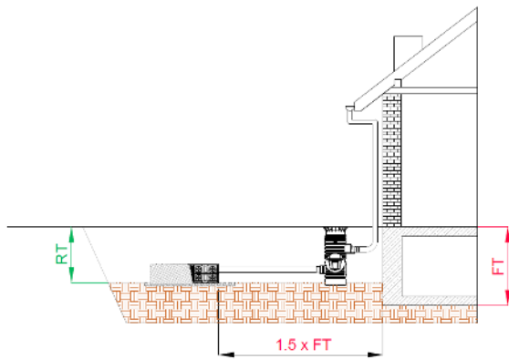
Figure 1: Installation situation: Foundation deeper than infiltration ditch module
