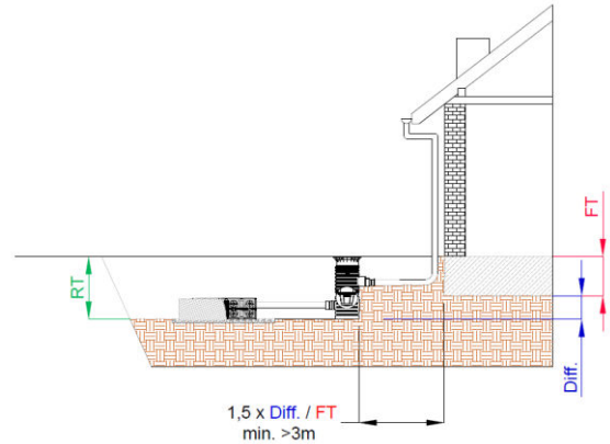
Figure 2: Installation situation: Infiltration ditch module deeper than the foundation
