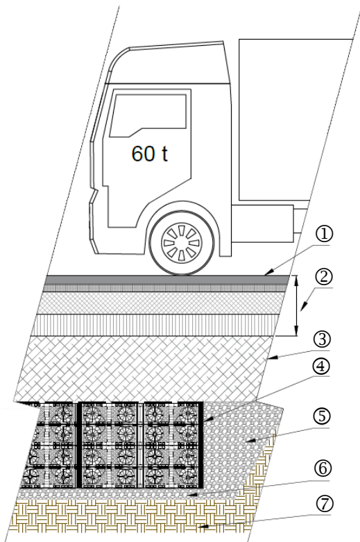
Figure 20: Installation under traffic areas up to HGV60
