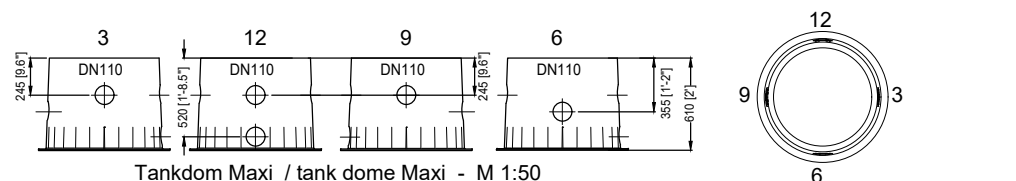
Tankdom Maxi / tank dome Maxi - M 1:50
